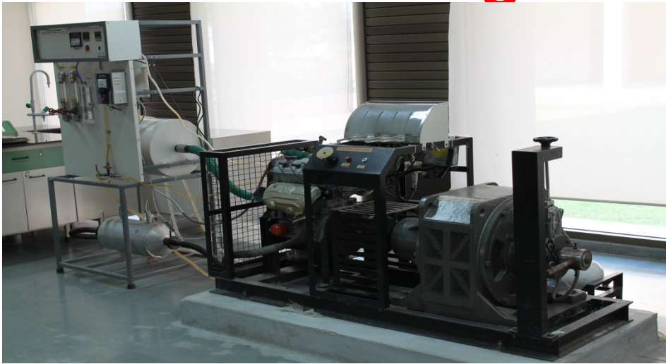
I C ENGINE , Eddy-current Dynamometer
