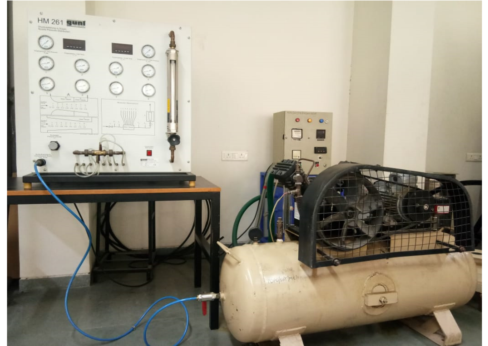
Nozzle Pressure Distribution System
